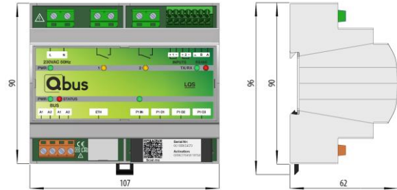
Figure 10 Dimensions LQS06SA
